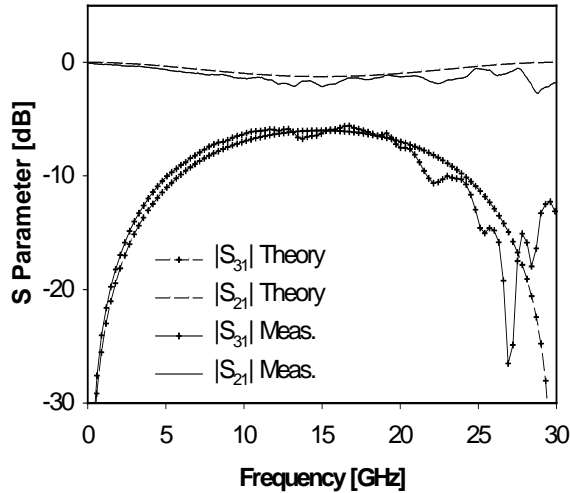
Fig. 3(a). Thru ( S_{21} ) and coupled ( S_{31} ) magnitude responses for a 6-dB CPW coupled-line device.
