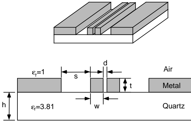
Fig. 1. Cross-section schematic of the CPW coupled-line geometry with dimension labels.
