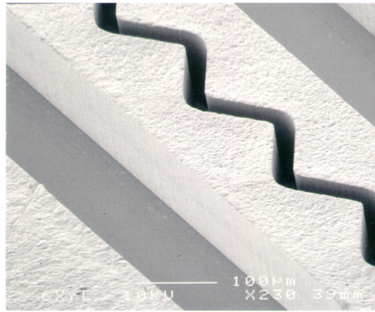
Fig. 4(b). SEM micrograph of 3-dB coupled lines in thick-metal single-section filter.
