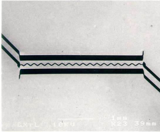
Fig. 4(a). SEM micrograph of a microfabricated thick-metal single-section CPW BPF.
