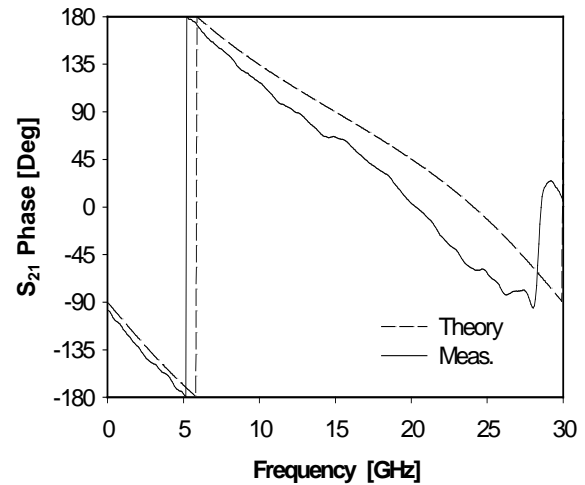
Fig. 5(b). Thru ( S_{21} ) phase response for a 3-dB coupled-line filter section.
